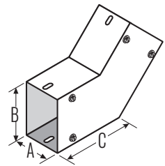
45° Elbow/Type C
